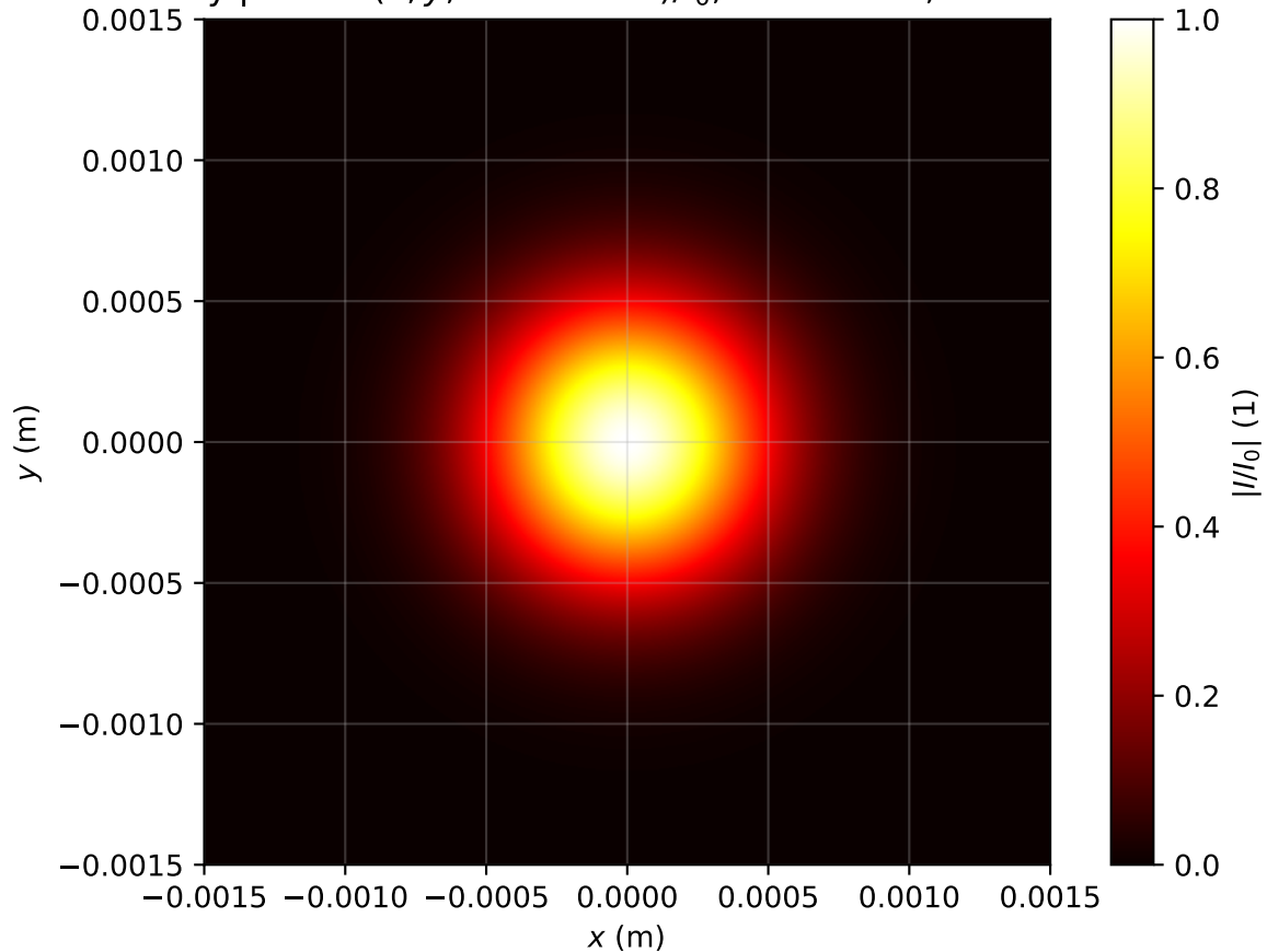
Intensity profile I(x, y, z = 0.000\text{m})/I_0 , \text{Pin}=0.2\text{Pcr} , artificial time
